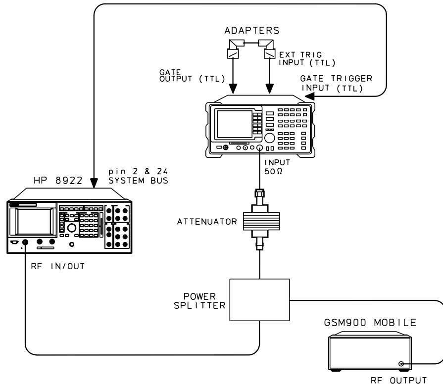
Figure 7 Triggering Connections using the HP 8922
