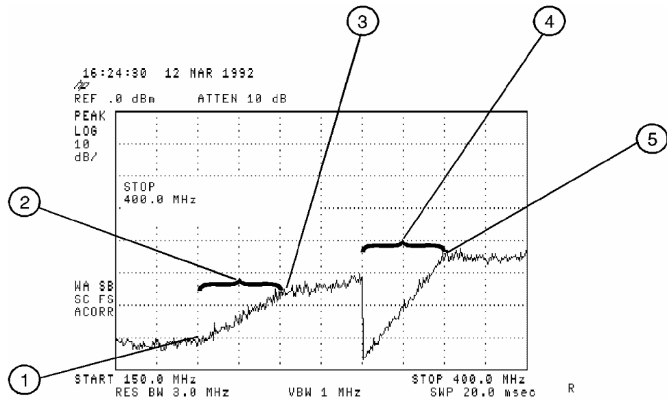
Figure 43 Amplitude-Correction Points
