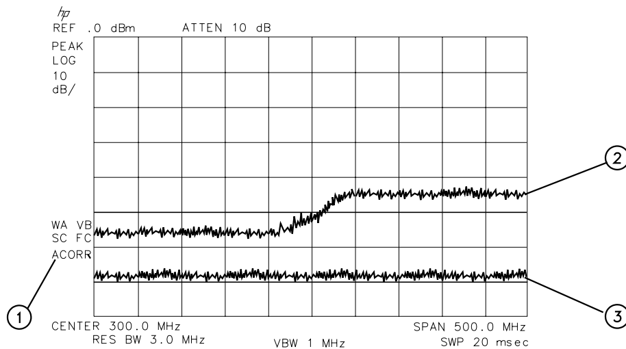
Figure 41 Amplitude-Correction Display
