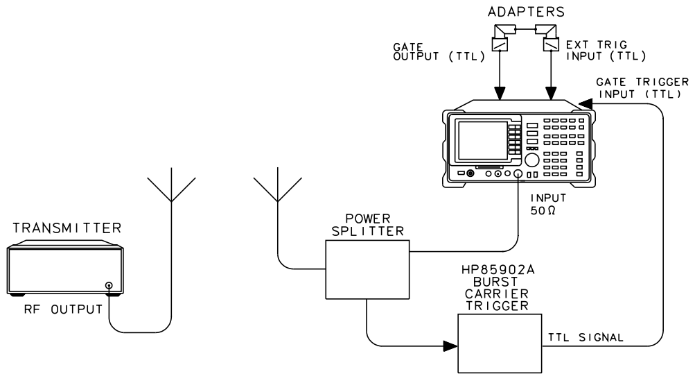
Figure 6 Triggering Connections using the HP 85902A and a Power Splitter
